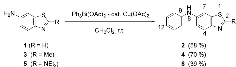
Scheme 2. Phenylation of 6-aminobenzothiazole derivatives 1 , 3 and 5
