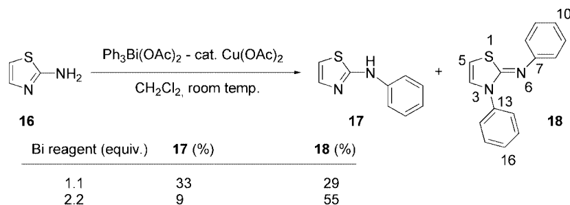
Scheme 4. Phenylation of 2-aminothiazole ( 16 )
