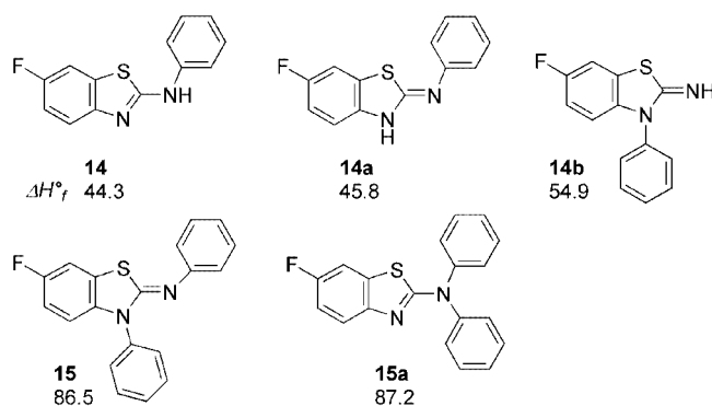
Scheme 5. Enthalpies of formation \Delta H_f^0 ( \text{kcal}\cdot\text{mol}^{-1} ) of different isomers of 14 and 15 after geometry optimisation by AM1 (RHF) semi-empirical calculations
