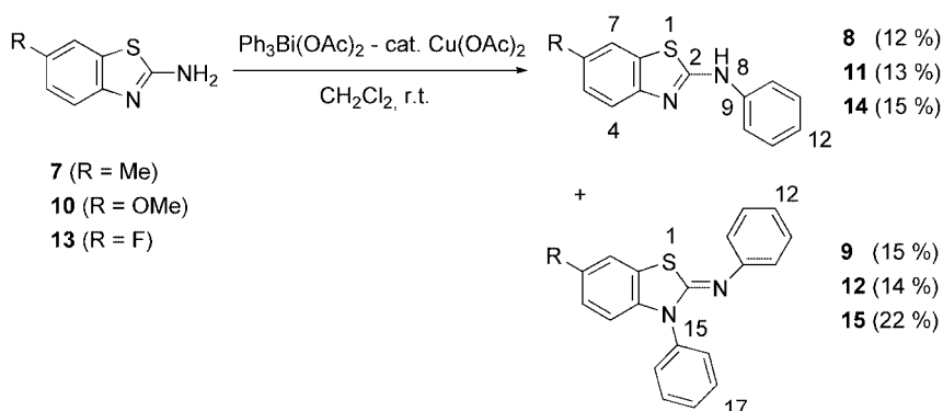
Scheme 3. Phenylation of 2-aminobenzothiazole derivatives 7 , 10 and 13
