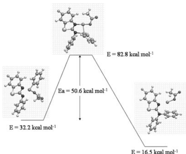
Scheme 9. Reaction pathway for the formation of 15a : second phenylation on the exocyclic nitrogen atom
