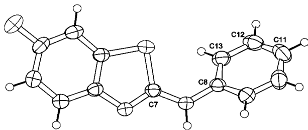
Figure 1. ORTEP view of compound 14
