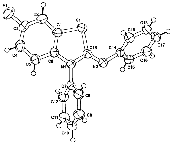
Figure 2. ORTEP view of compound 15
