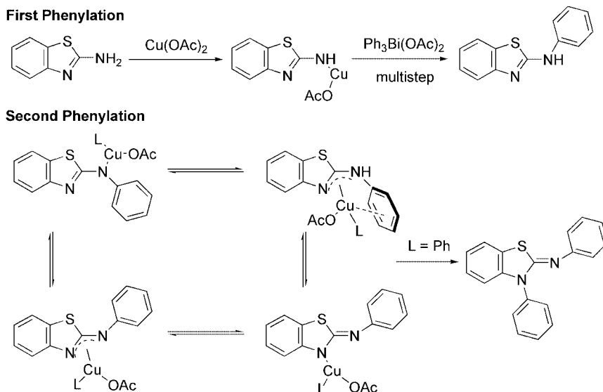
Scheme 6. Plausible copper intermediates involved in the ligand-transfer step
