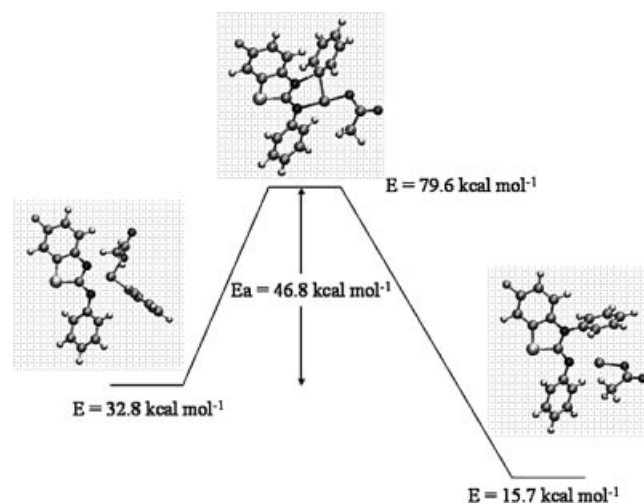
Scheme 8. Reaction pathway for the formation of 15 : second phenylation on the endocyclic nitrogen atom
